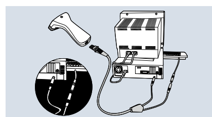
Tastaturemulation
