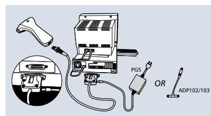
RS232
